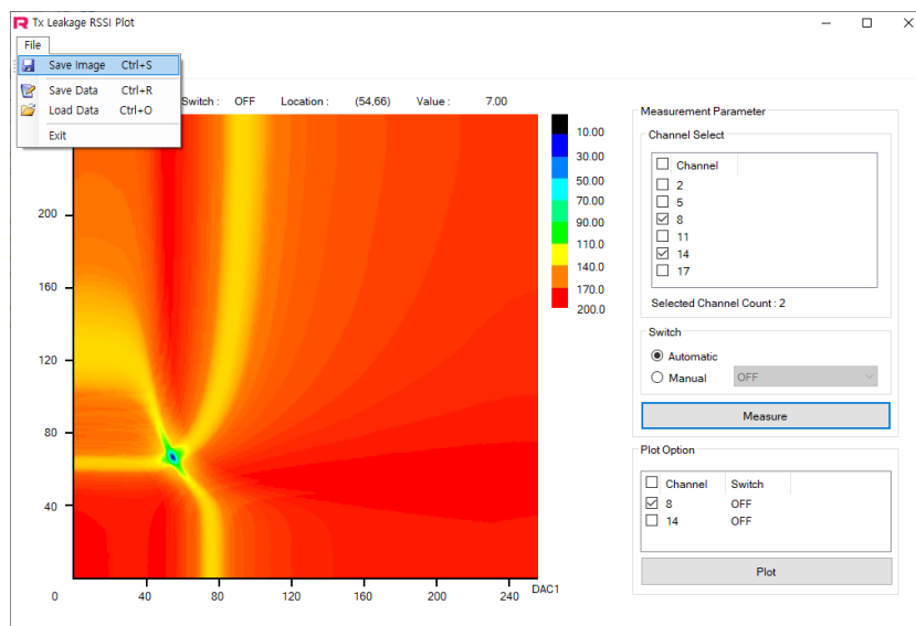
Figure 60 Save Raw Data
